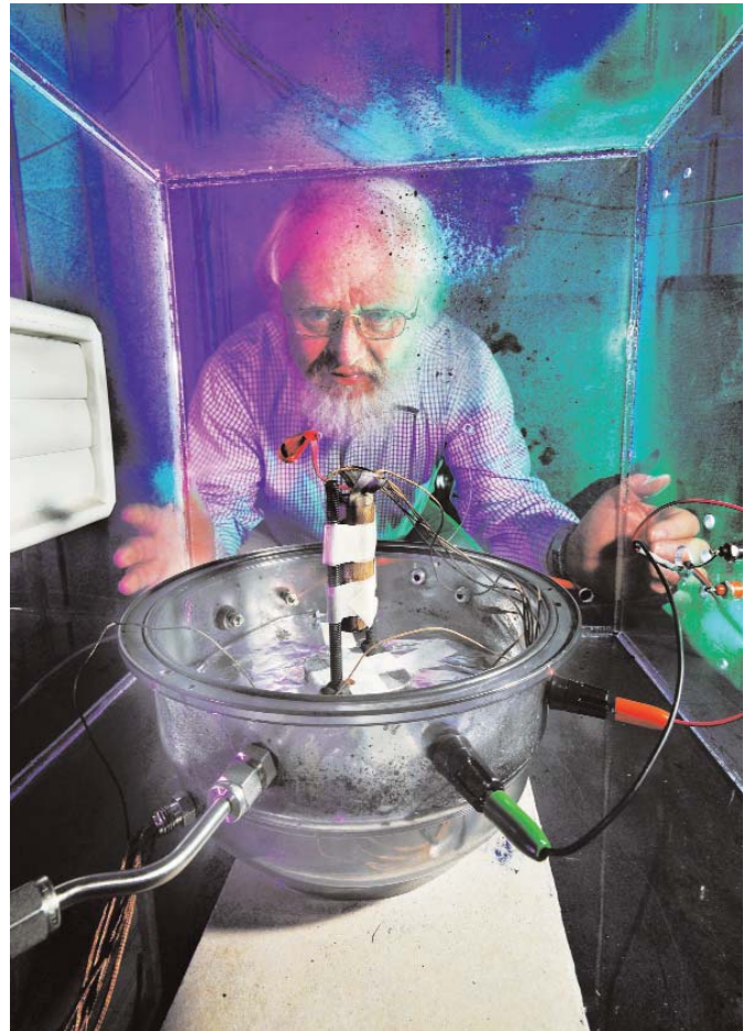
Sandia researcher Peter Roth prepares to blow up a battery to see how robust it is. The work is part of the DOE-funded FreedomCAR program.
