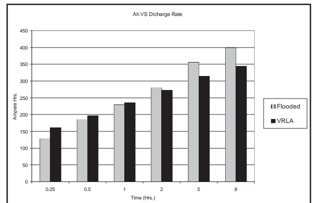
Figure 1. AH VS discharge rate for flooded and VRLA (400 Ah @ C/8)
